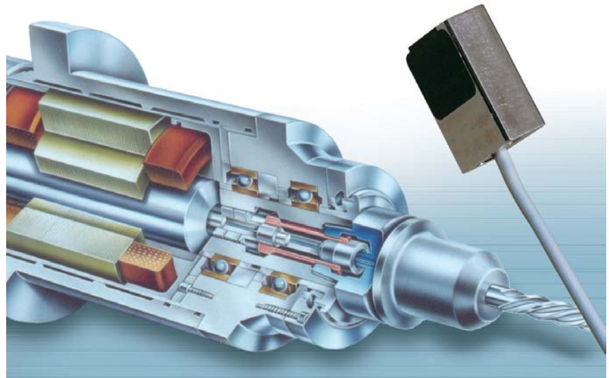
An internal sensor solution that can be reused and requires no recalibration
