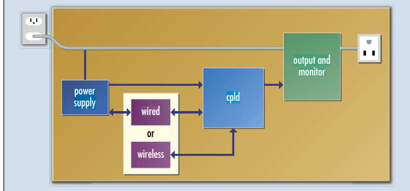
Figure 1: A typical local device controller
