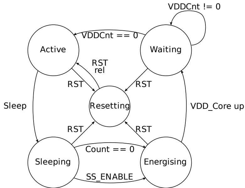
Figure 5 PCU state diagram
