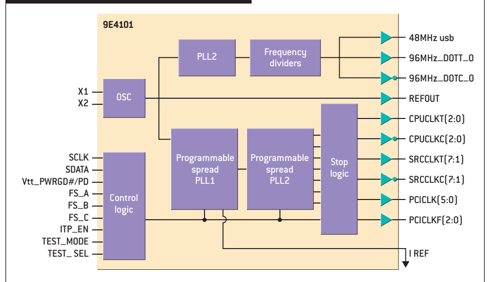
Fig 1: Block diagram of the 9E4104 embedded clock
