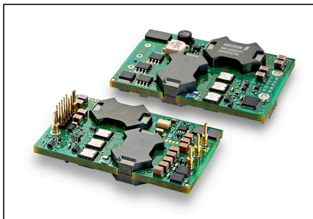
Figure 3 - BMR453 top and bottom view
