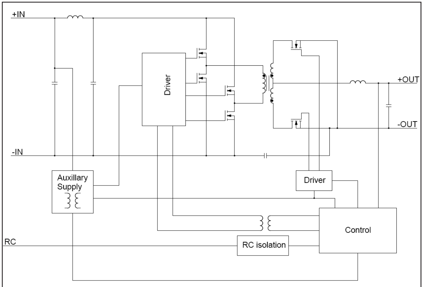
Figure 4 - BMR453 block diagram
