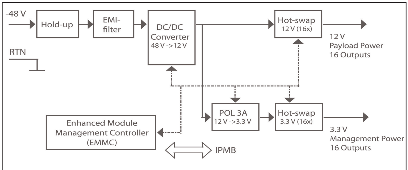
Figure 2 - MicroTCA power module block diagram
