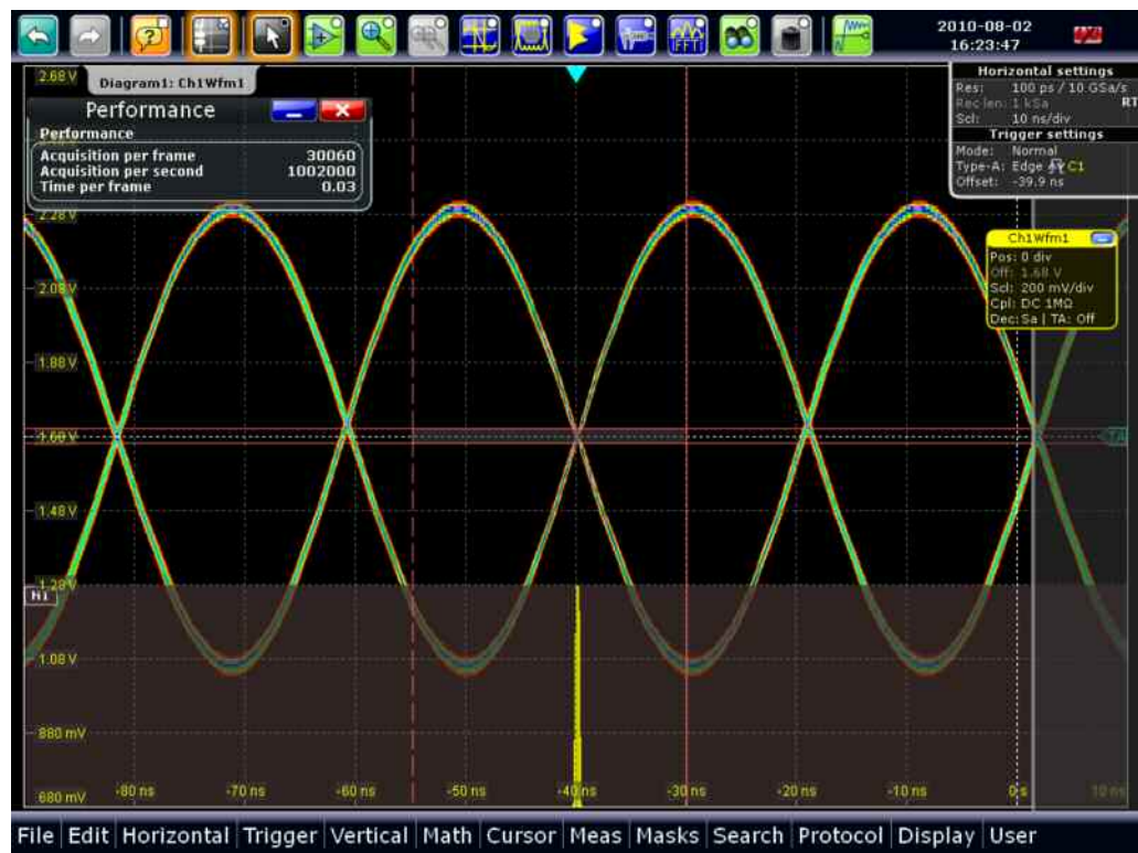
Figure 11: The high acquisition rate even with FFT provides a lively spectrum display
